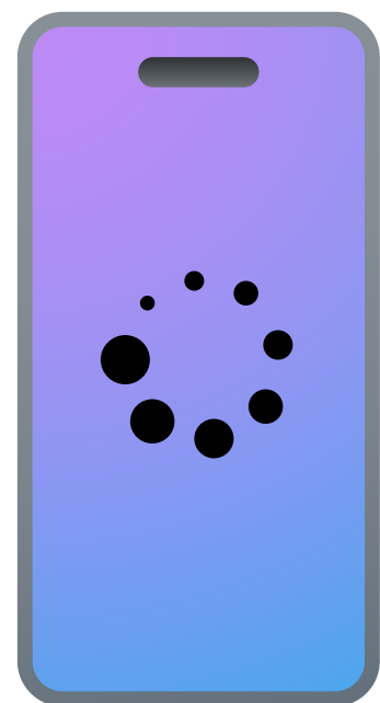
App
